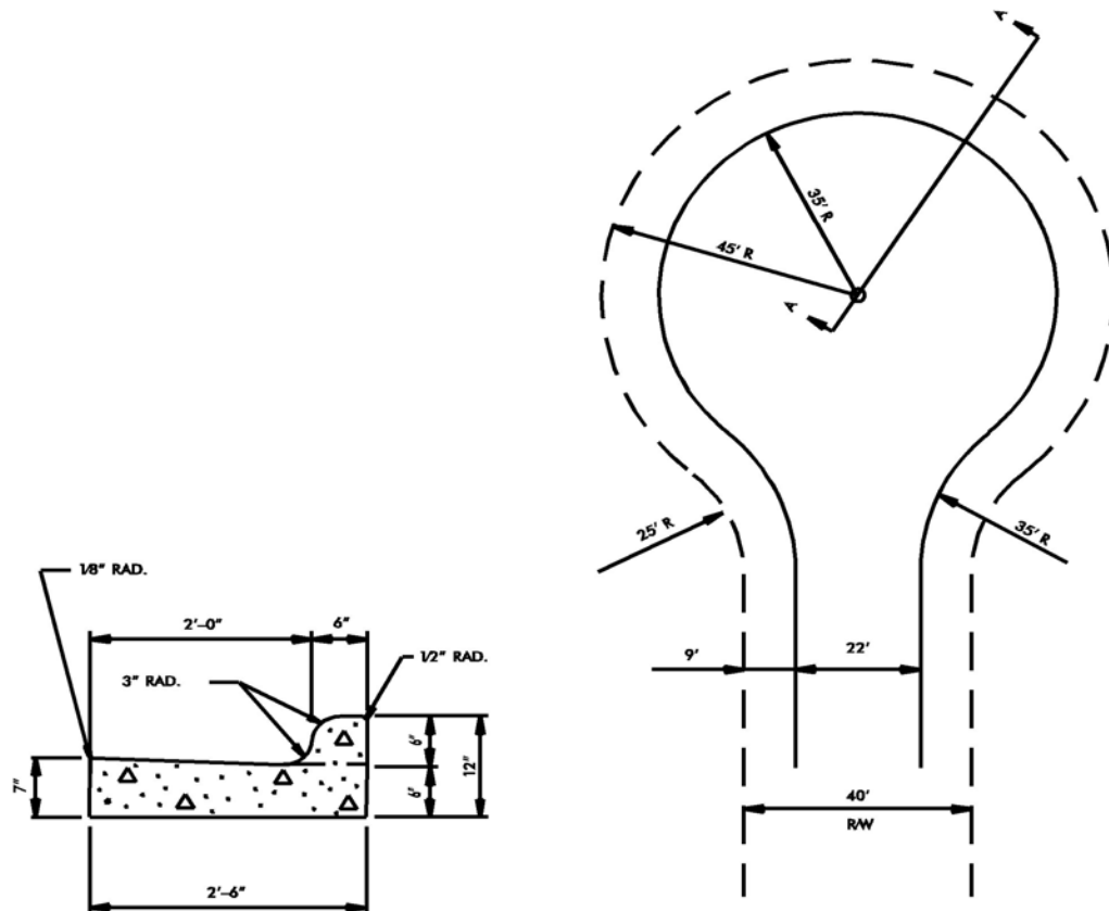
2'-6" CURB & GUTTER
